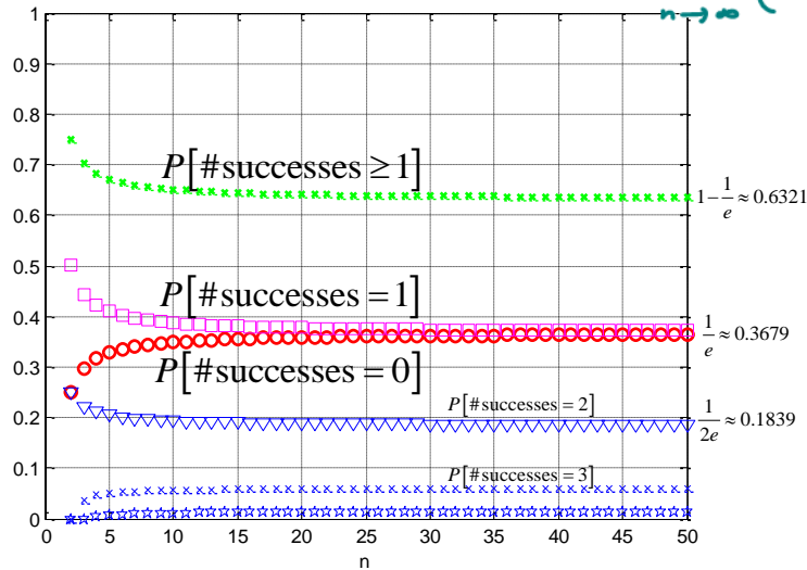
Figure 11: Number of occurrences of 1-in- n -chance event in n repeated Bernoulli trials
